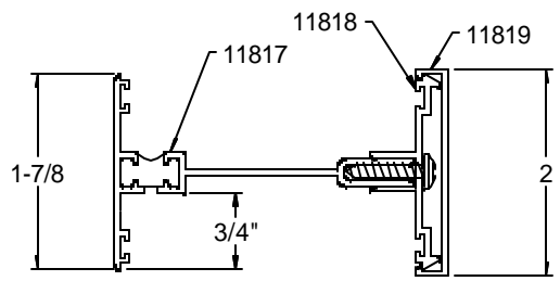
3 Piece Mullion
