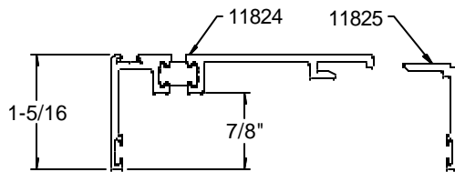
2 Piece Receptor
