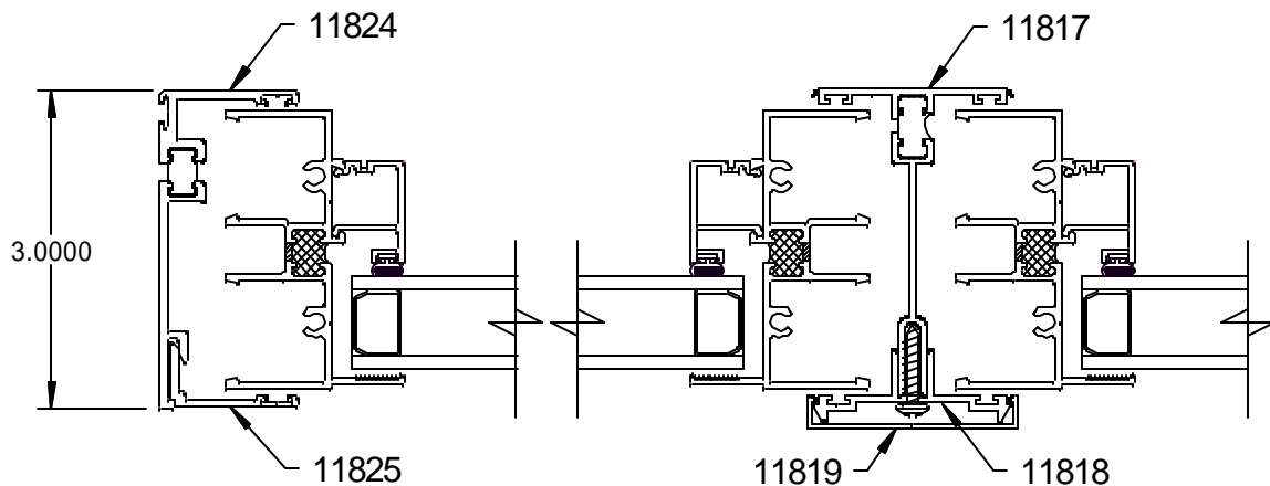
Fixed Window with 2 Piece Receptor and 3 Piece Vertical Mullion
