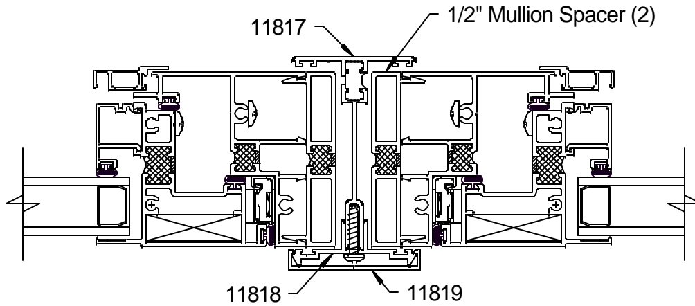
Projected (Casement) with 3 Piece Vertical Mullion and 1/2" Mullion Spacers
