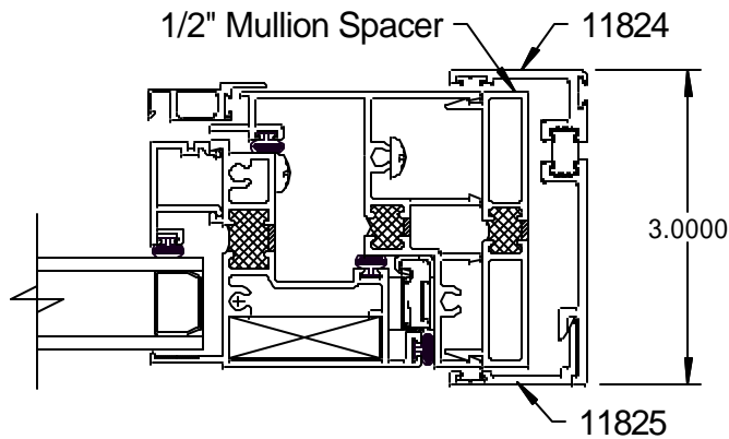
Projected (Casement) with 2 Piece Receptor and 1/2" Mullion Spacer
