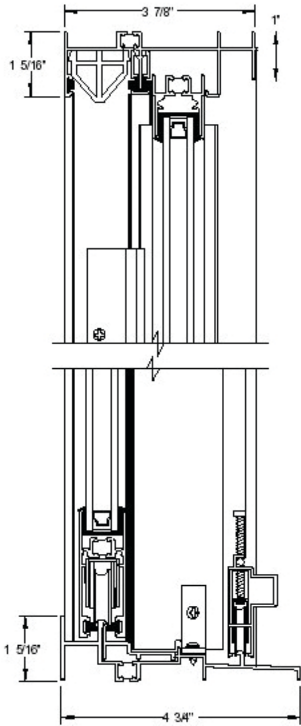
Cross Section
